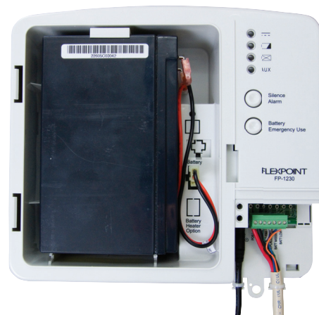
FlexPoint 1230 Shown with cover removed, battery, auxiliary power cable and NID hook-up cable
